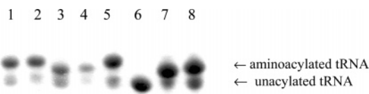
Figure 3. Analysis of protected aminoacylated tRNA Phe C UA by electrophoresis on an acidic 8% polyacrylamide–7 M urea gel. Lane 1, 2,3,4,6-tetra- O -acetyl-β- D -galactosylseryl-tRNA; lane 2, 2,3,4,6-tetra- O -acetyl-β- D -glucosylseryl-tRNA; lane 3, β- D -galactosylseryl-tRNA; lane 4, tyrosyl-tRNA; lane 5, 4- O -(β- D -galactopyranosyl)-β- D -glucopyranosyltyrosyl-tRNA; lane 6, unacylated tRNA; lane 7, β- D -glucosyltyrosyl-tRNA; lane 8, β- D -galactosyltyrosyl-tRNA.
